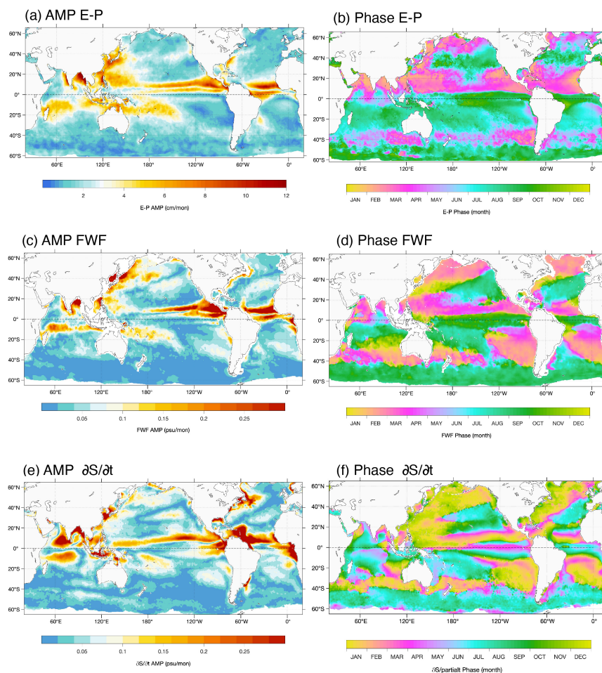
Figure 5. Amplitude-phase asymmetry in seasonal salinity variability demonstrates forcing sets variance amplitude but circulation determines spatial-temporal distribution. Harmonic analysis of (a,b) atmospheric freshwater forcing E-P , (c,d) freshwater flux FWF = S_0(E-P)/h , and (e,f) observed salinity tendency \partial S/\partial t from satellites (2010-2020). Left panels show seasonal amplitude; right panels show phase (month of annual maximum). Adapted from Yu et al. (2021).
