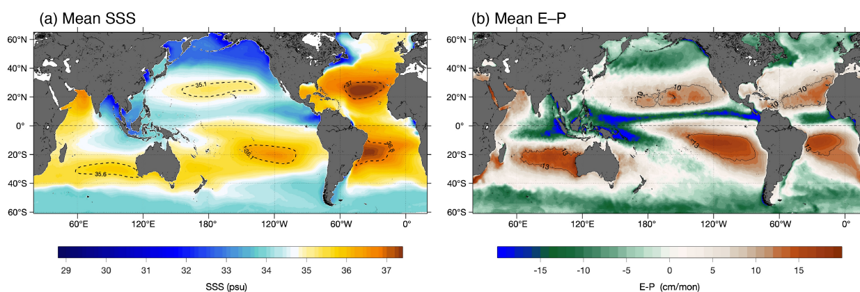
Figure 1. Time-mean fields. (a) sea surface salinity (SSS) and (b) evaporation minus precipitation (E – P) averaged over 2012-2022. Adapted from Yu (2023).
