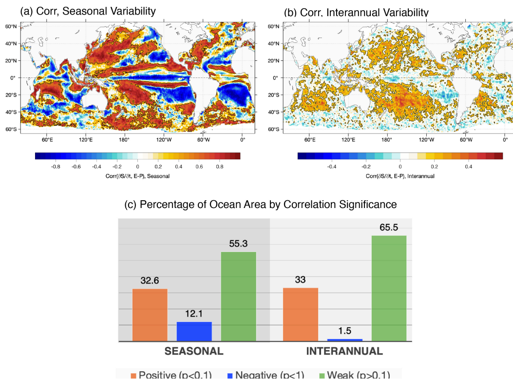
Figure 3. Correlation between E-P and \delta S/\delta t at seasonal and interannual timescales (2012-2022). Spatial distribution of correlation coefficients for (a) seasonal variability (demeaned) and (b) interannual variability (detrended and deseasonalized). (c) Percentage of ocean area showing statistically significant positive correlations ( p < 0.1 , orange), significant negative correlations ( p < 0.1 , blue), and weak, non-significant correlations ( p > 0.1 , green). Significant positive correlations occupy 33% of ocean area at both timescales, while weak correlations dominate (55% seasonal, 66% interannual). Correlation thresholds for significance ( p < 0.1 ) are 0.50 for seasonal and 0.14 for interannual variability. Adapted from Yu et al. (2021).
