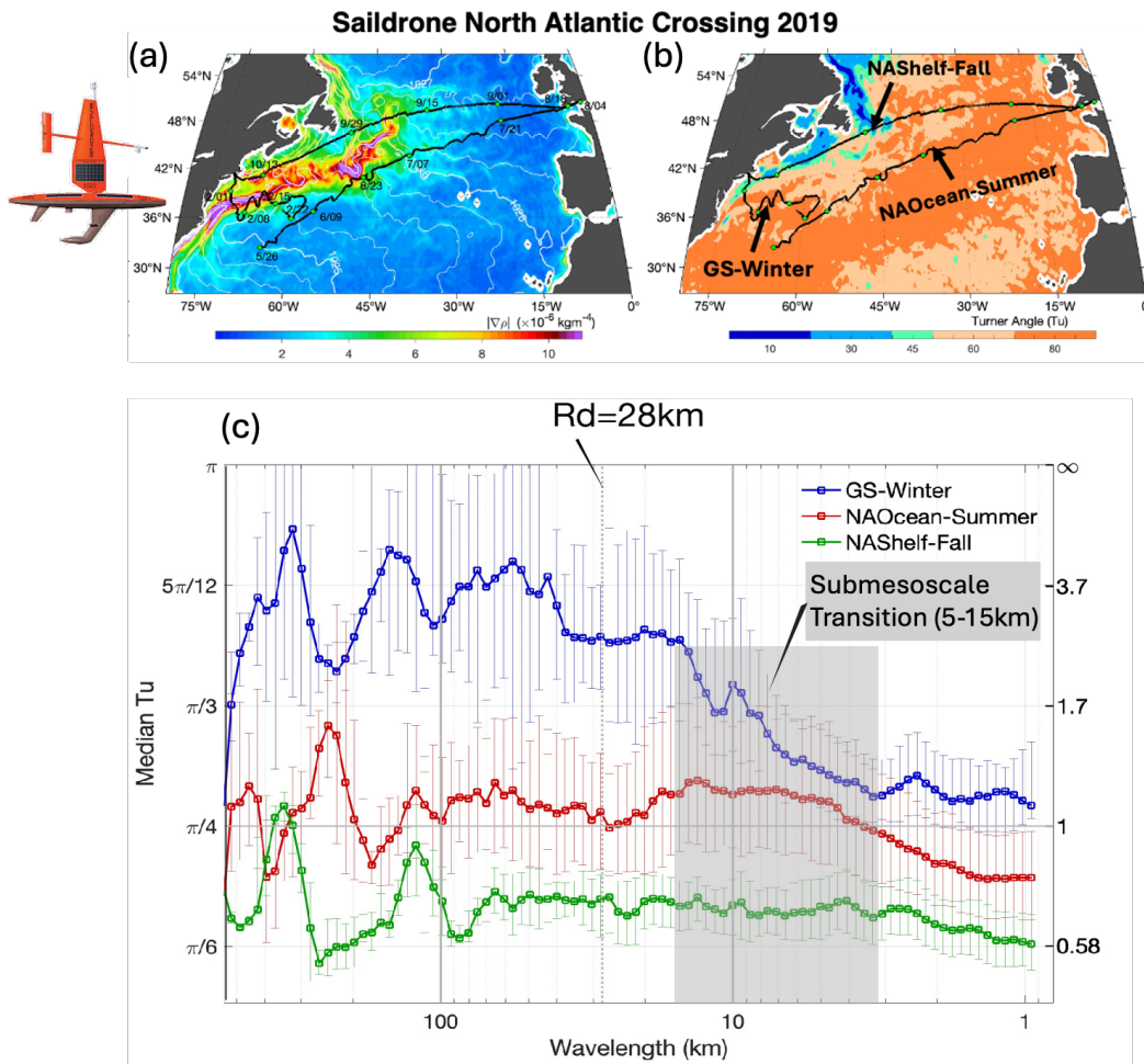
Figure 7. Thermohaline regime transition at submesoscales. (a) Sea surface density gradient magnitude and (b) Turner angle ( Tu ) from satellite observations with 2019 North Atlantic Saildrone tracks overlaid (black lines). Tu less than 45^\circ (blue) indicates salinity-dominated density; Tu greater than 45^\circ (orange) indicates temperature-dominated density. (c) Median Turner angle (left axis) and density ratio R\rho (right axis) versus wavelength computed from Saildrone measurements for three regimes: Gulf Stream winter (blue), open ocean summer (red), and continental shelf fall (green). Dashed line marks deformation radius ( R_d = 28 \text{ km} ); gray shading indicates submesoscale transition zone (5-15 km); horizontal line marks Tu =
