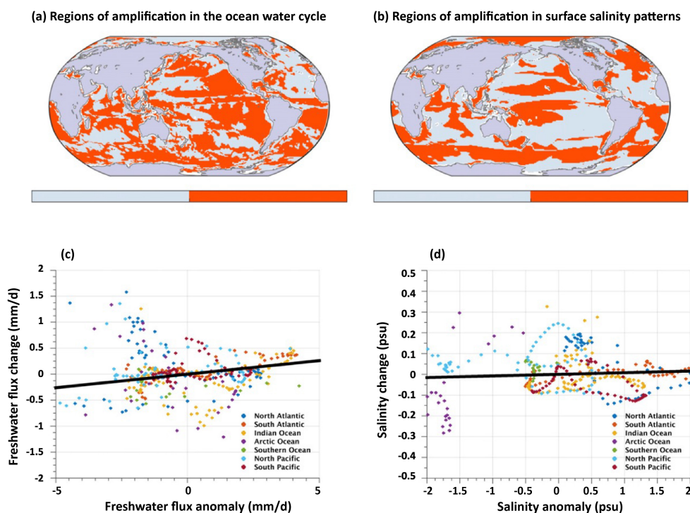
225 Figure 4. Pattern amplification in ocean water cycle versus surface salinity over 1993-2010. (a,b) Regions where climatological patterns amplified (orange: wet regions got wetter and dry regions got drier for freshwater flux; fresh regions got fresher and salty regions got saltier for salinity) versus weakened (gray). (c,d) Strength of pattern amplification: x-axis
